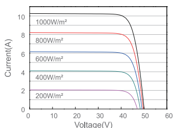
Current-Voltage Curve M72D10-410/MB
