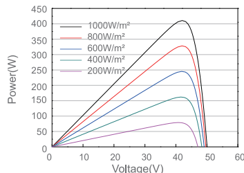
Power-Voltage Curve M72D10-410/MB
